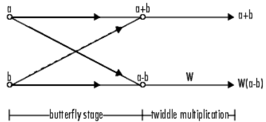
Decimation-in-frequency IFFT
